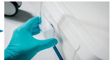
CATSmart vacuum line with integrated Hydrophobic filter
